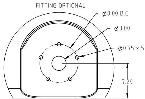
DETAIL B SCALE 2:25
