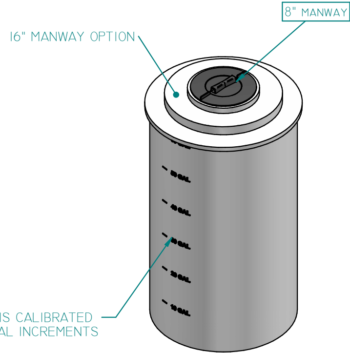
ISO VIEW
